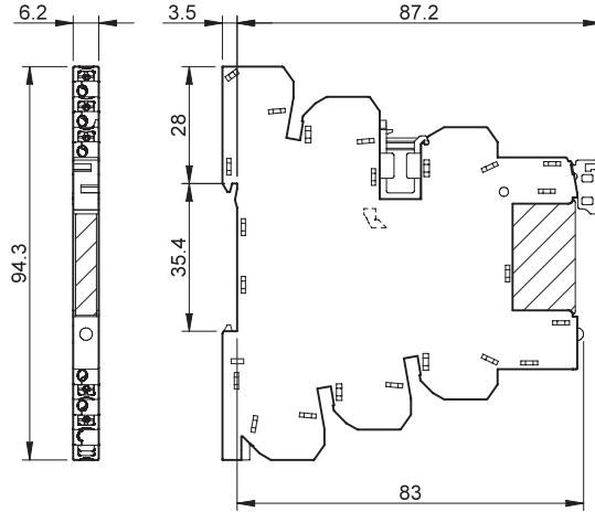
Tipo 39.90 39.91 Borne push-in
